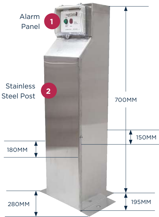
HIGH WATER LEVEL ALARM CONTROL BOX
