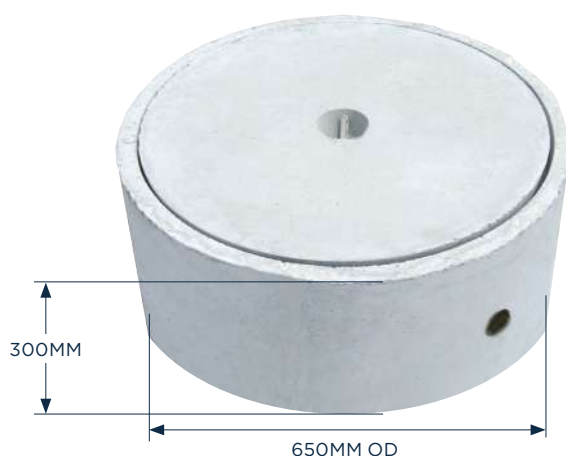
ABS/COMPACT RISER - 55KG
