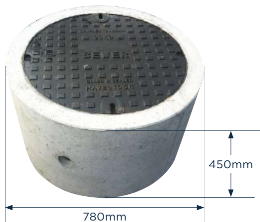
450MM RAINWATER TANK RISER WITH CLASS B GATIC ACCESS COVER - 100KG For Sewer and Stormwater
